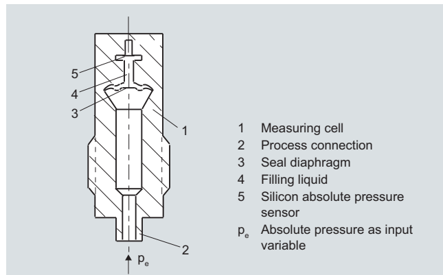
Measuring cell for absolute pressure from the pressure series, function diagram
